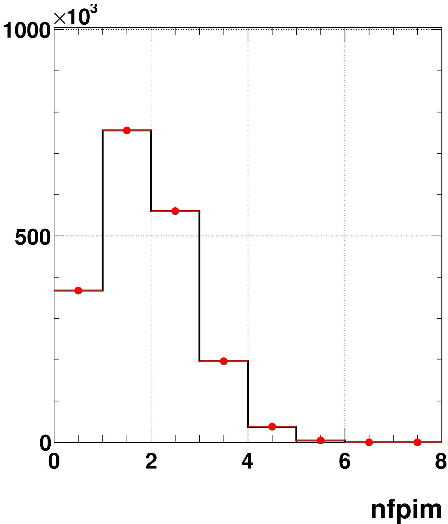
Number of final state pi- / DIS only
