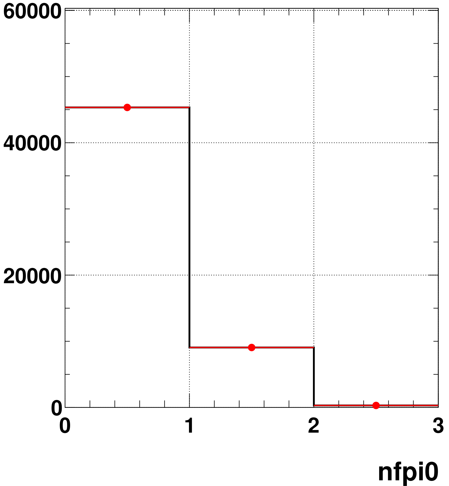
Number of final state pi0 / RES only
