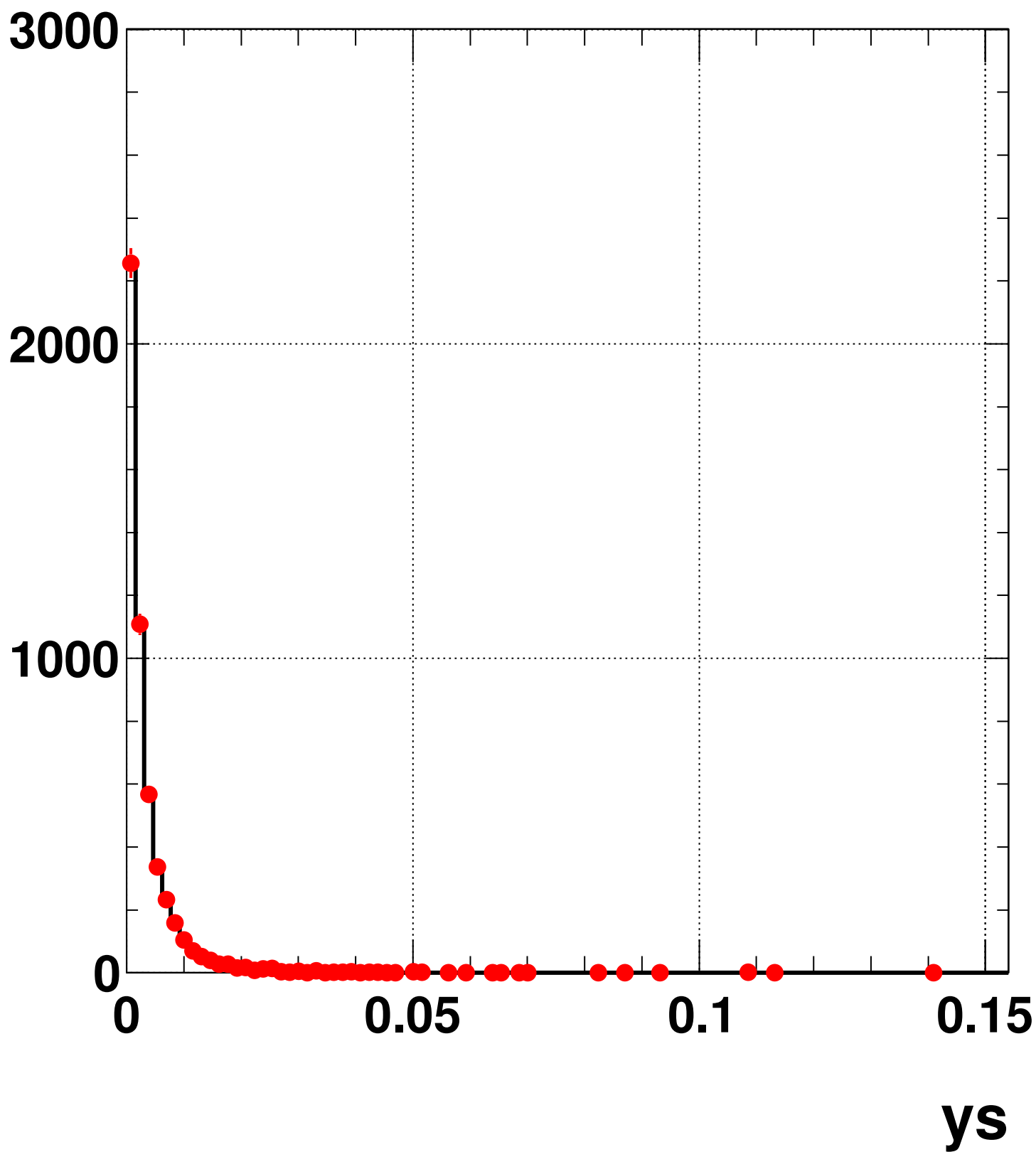
selected y for QEL events
