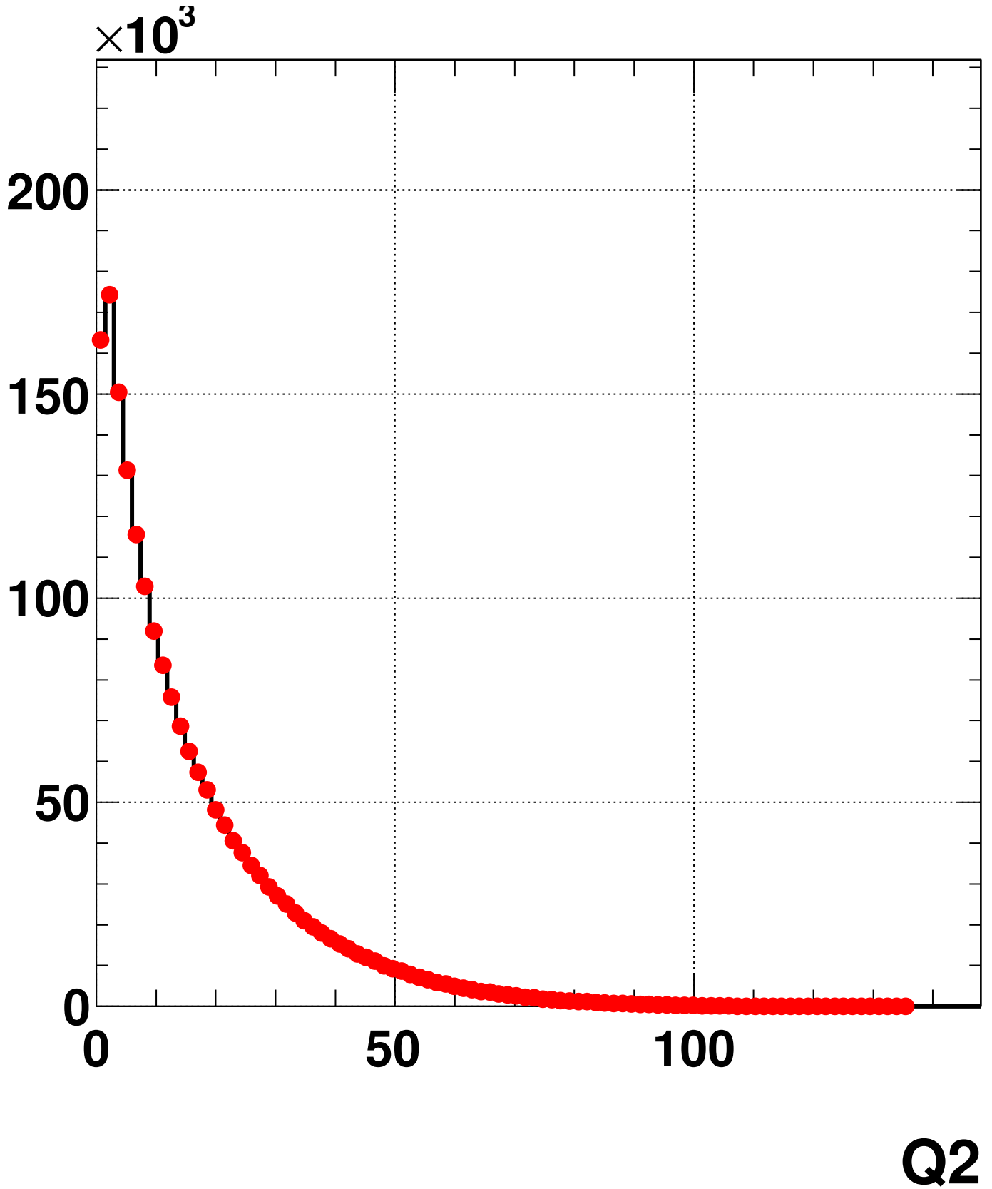
computed Q2 for DIS events
