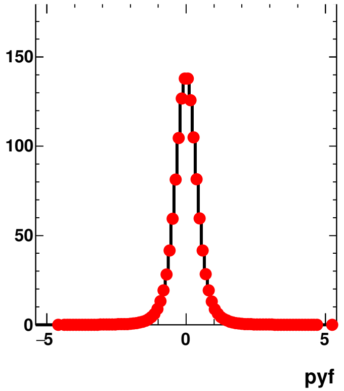
Final state protons 4-momentum / DIS only
