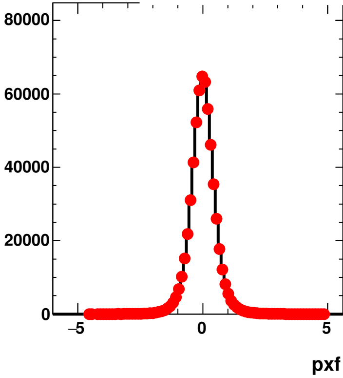
Final state neutrons 4-momentum / DIS only
