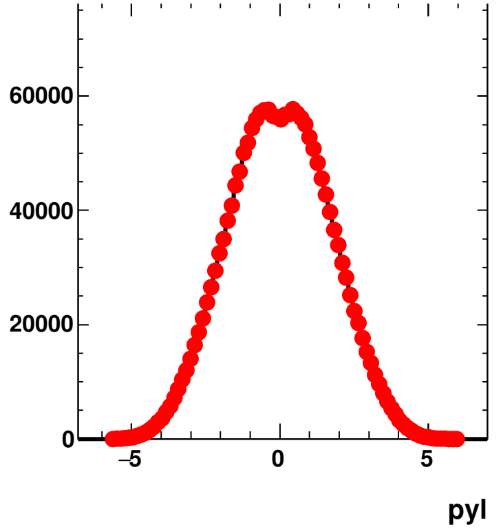
Final state primary lepton 4-p: All DIS events
