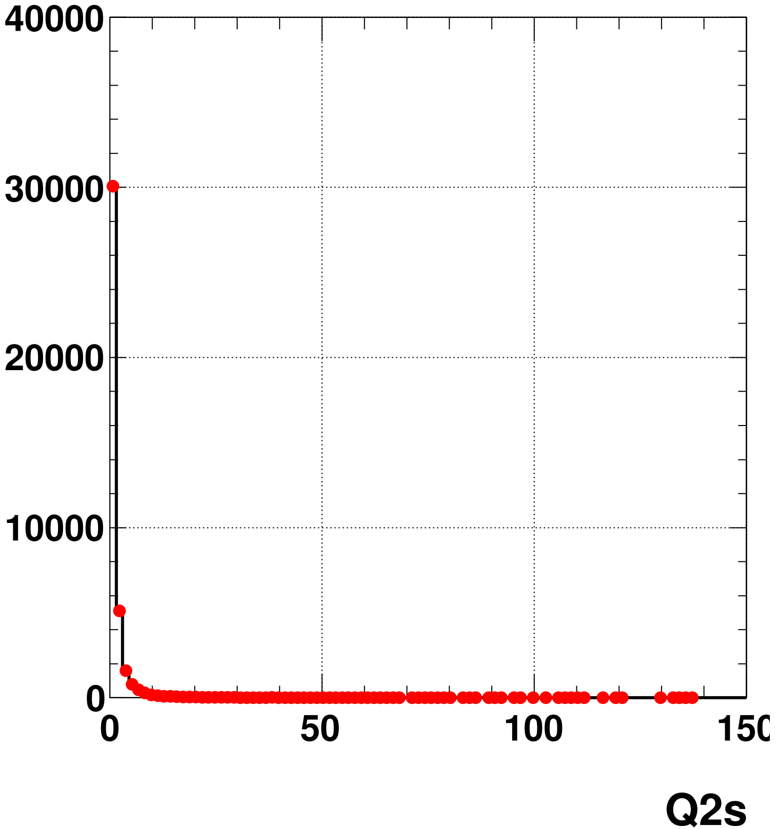
selected Q2 for RES CC events
