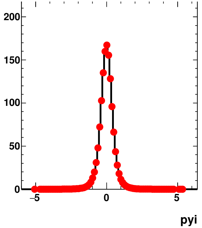
Primary Hadronic System: proton 4-momentum
