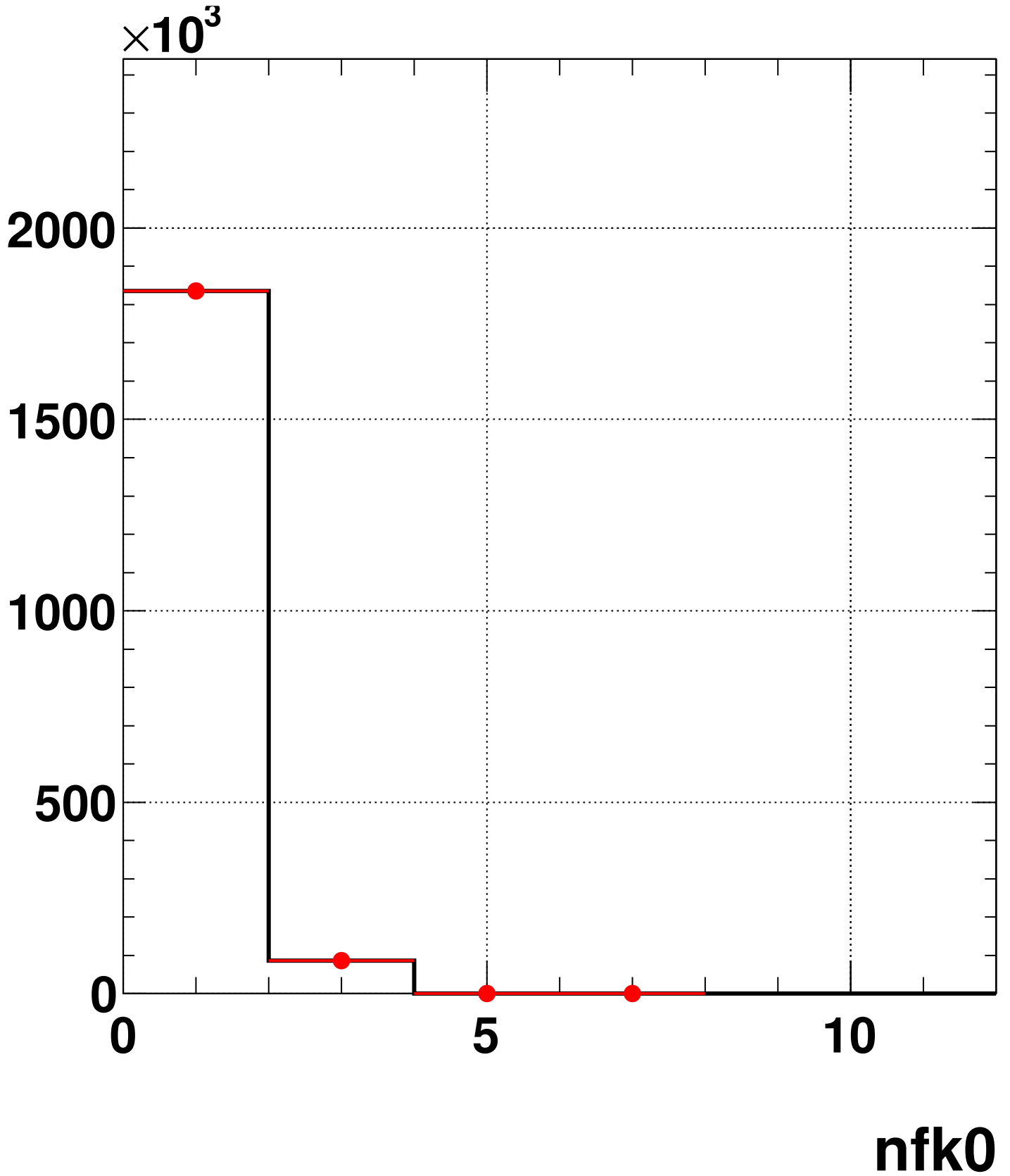
Number of final state K0 / DIS only
