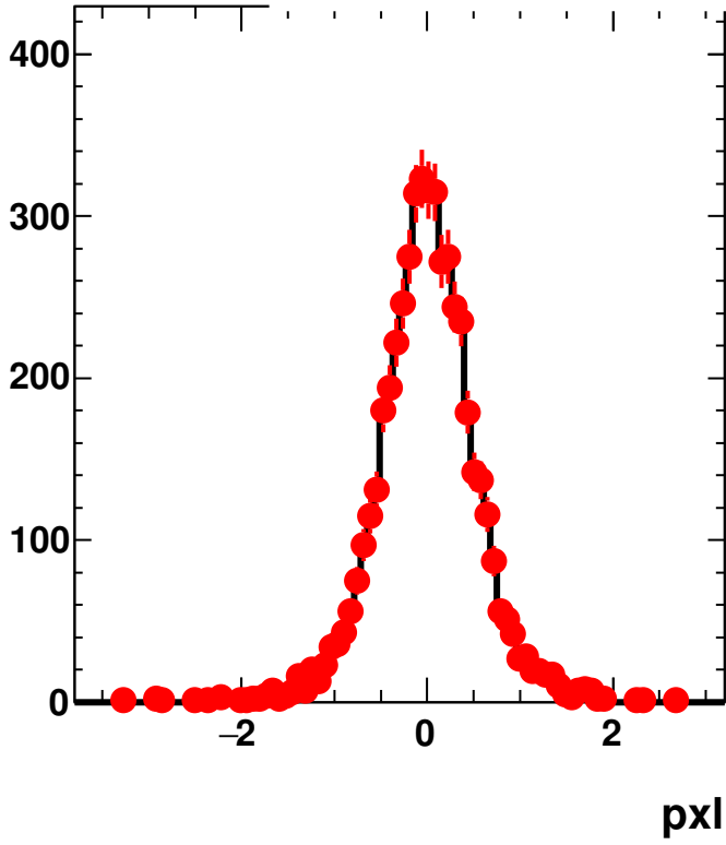
Final state primary lepton 4-p: QEL events
