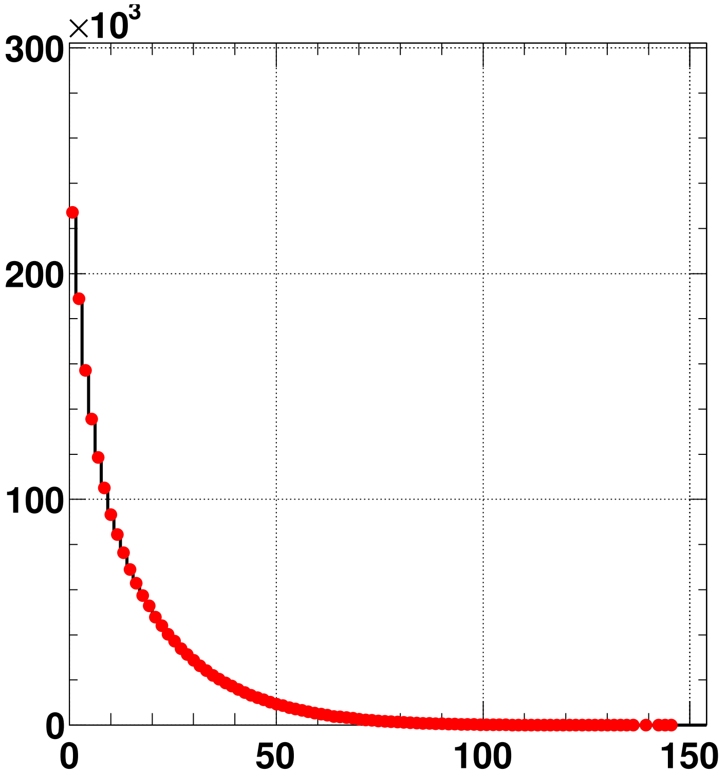
selected Q2 for all events
