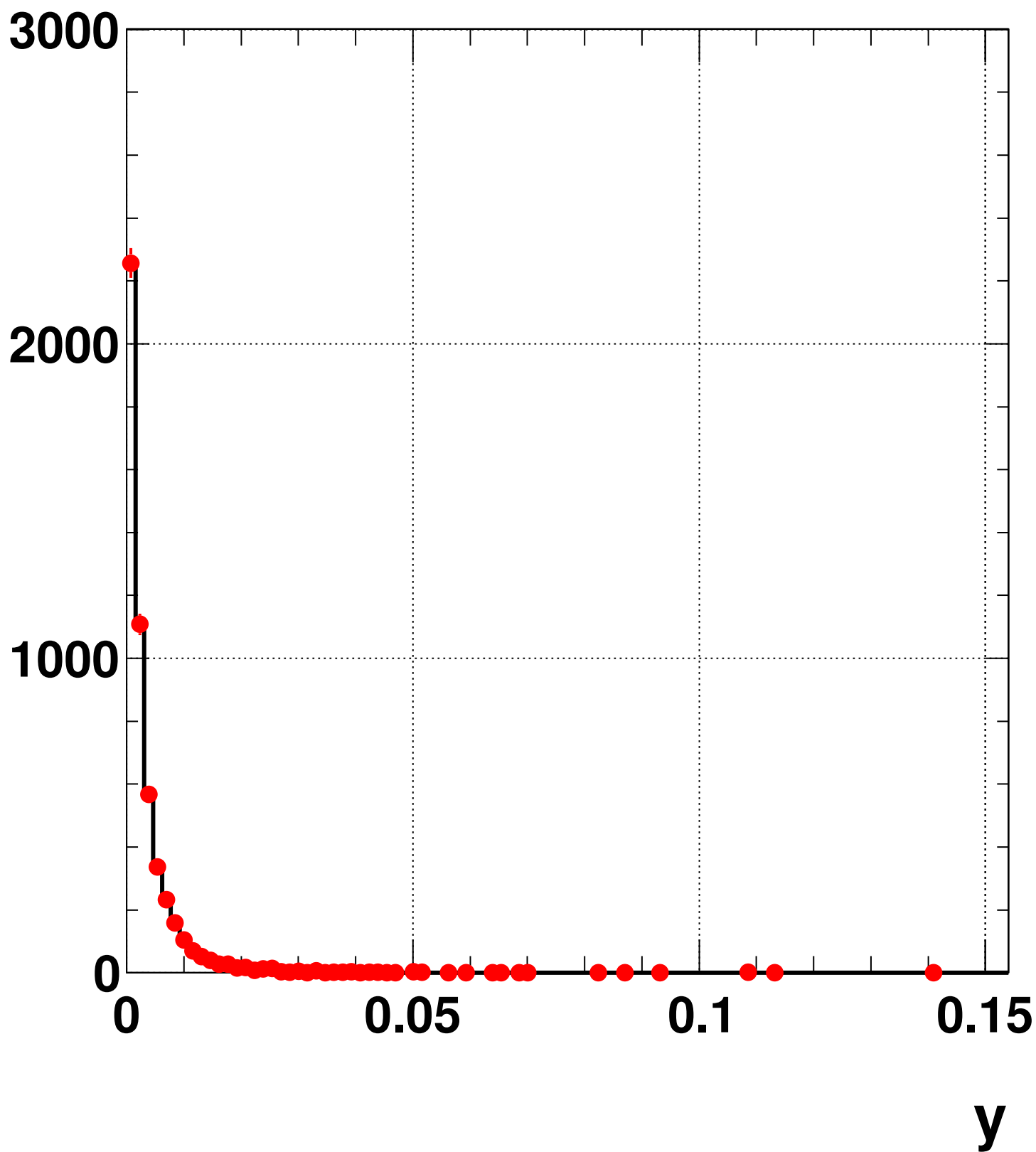
computed y for QEL events
