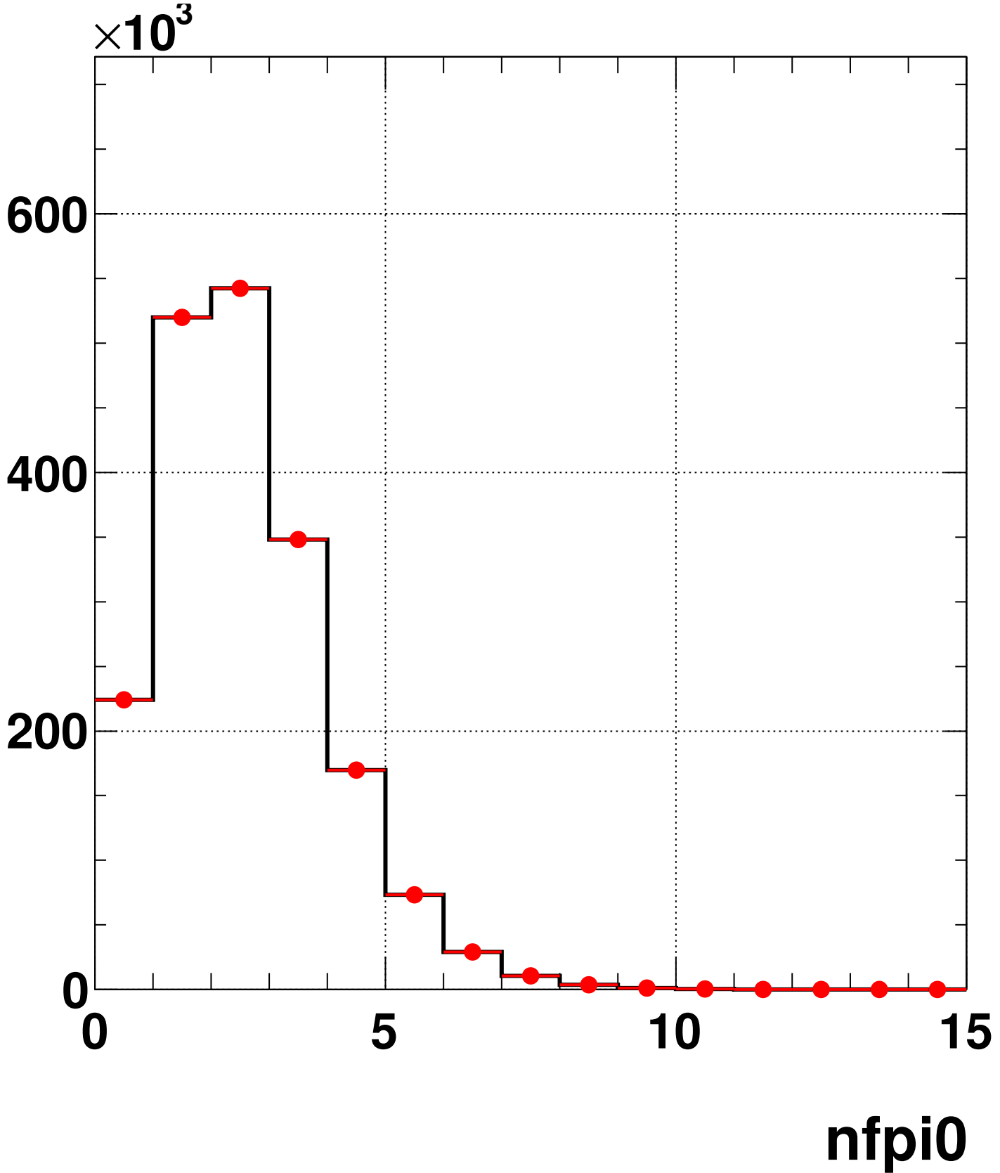
Number of final state pi0 / DIS only
