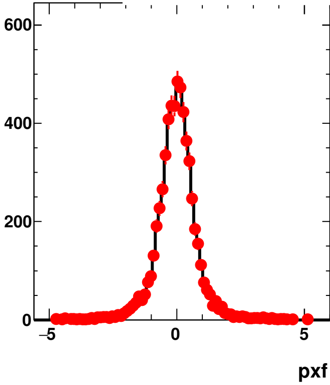
Final state neutrons 4-momentum / RES only
