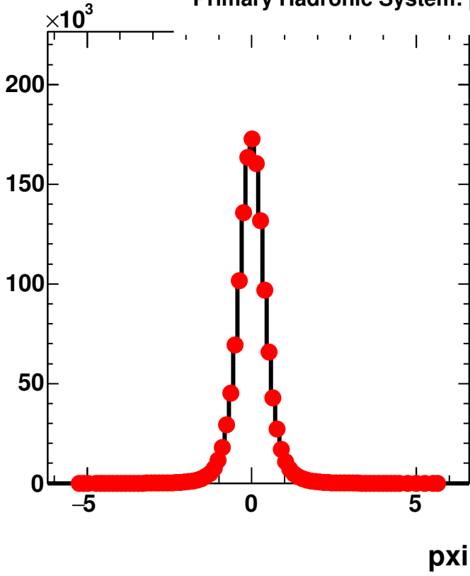
Primary Hadronic System: proton 4-momentum
