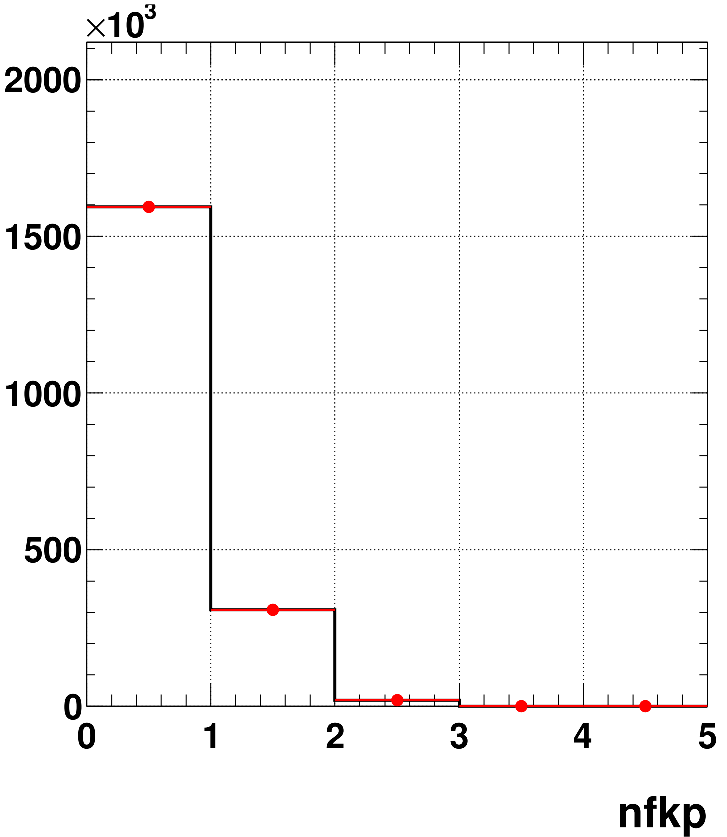
Number of final state K+ / DIS only
