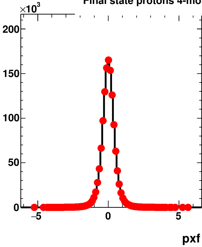
Final state protons 4-momentum / DIS only
